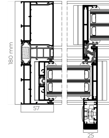
INTERLOCK HANDLE
