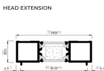
Head Extension 20 mm
