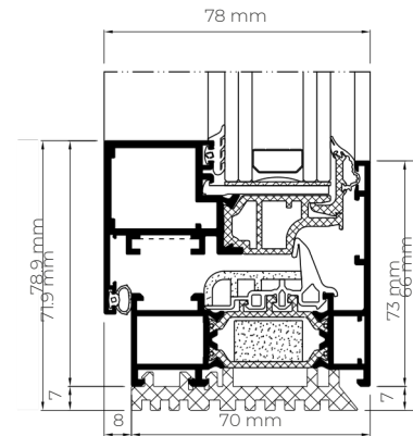
HIDDEN DRAINAGE
