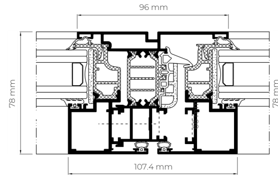
FLOATING MULLION
